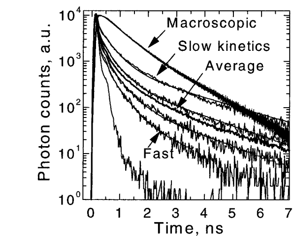
FIGURE 2 TCSPC traces from selected spots in various LHCII clusters of Fig. 1 and a TCSPC trace recorded in a macroscopic measurement. The average trace ( thick line ) was obtained by summing all the microscopic fluorescence decays measured in the same aggregate. Thin lines are multiexponential fits to the experimental traces. The fitting parameters of the labeled traces are shown in Table 1. The fastest kinetics is the instrument response of the microscopic measurement.
